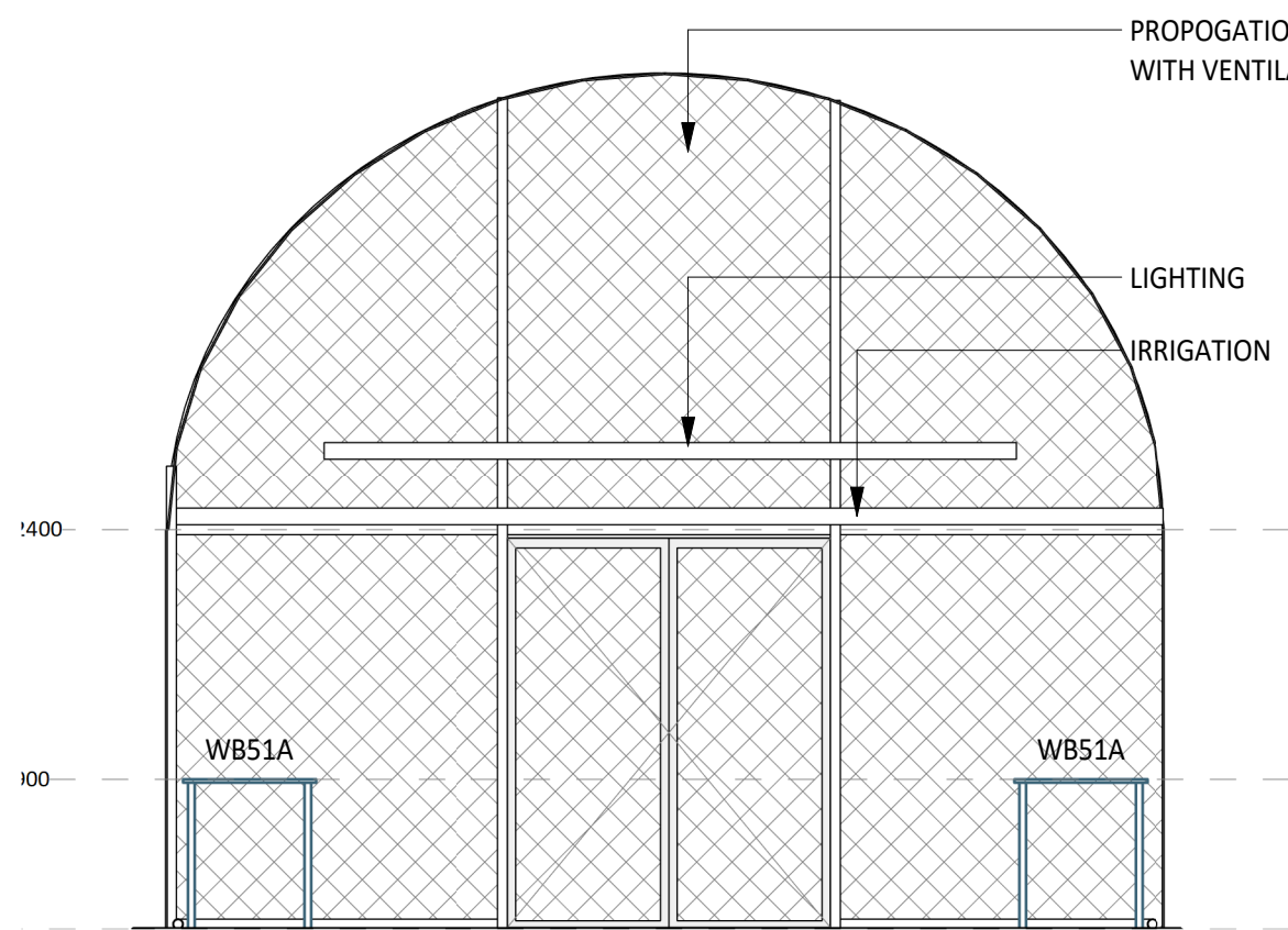
2 ELEVATION DETAIL 60-004 1 : 50
