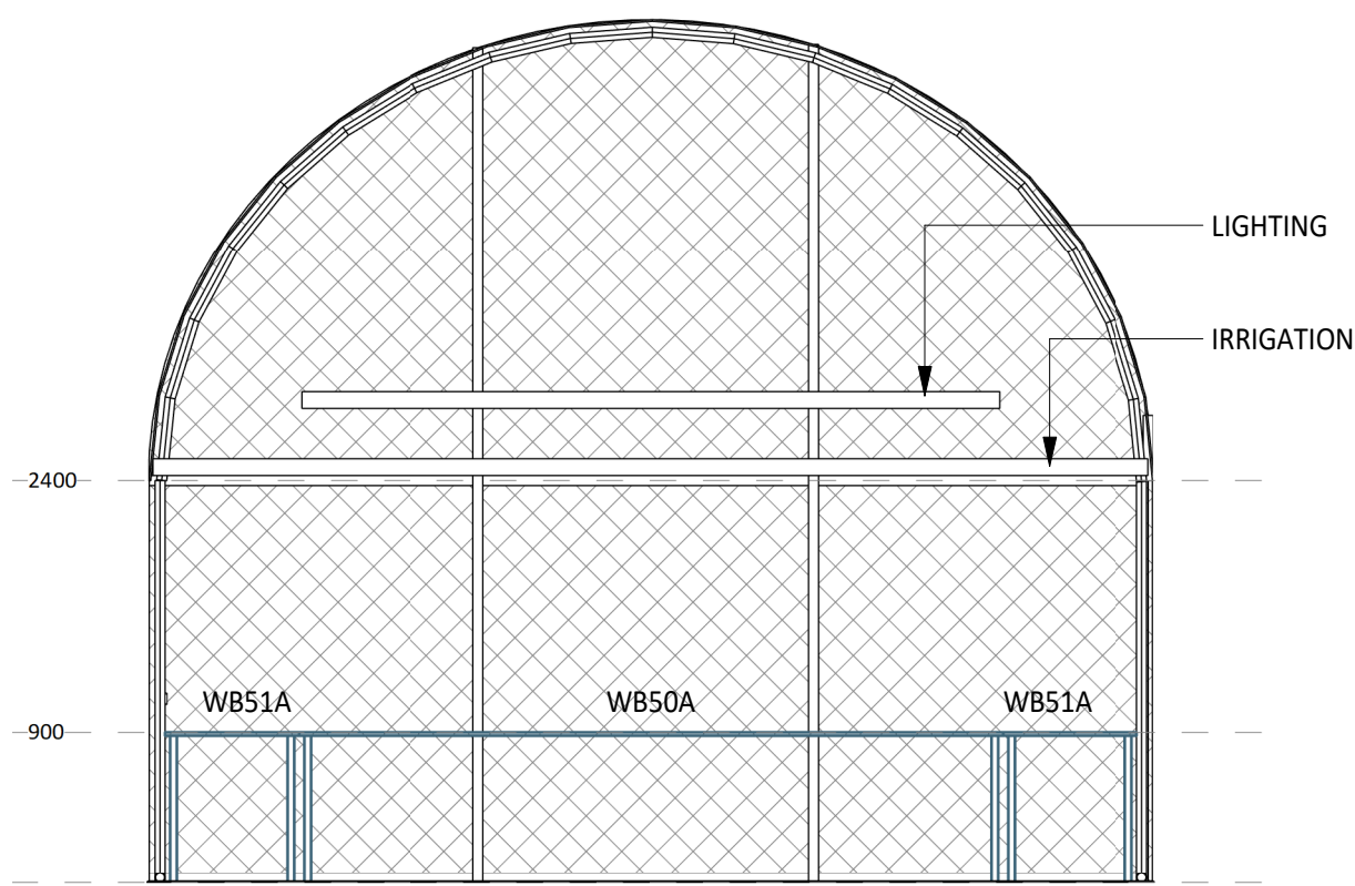
4 ELEVATION DETAIL 60-007 1 : 50
