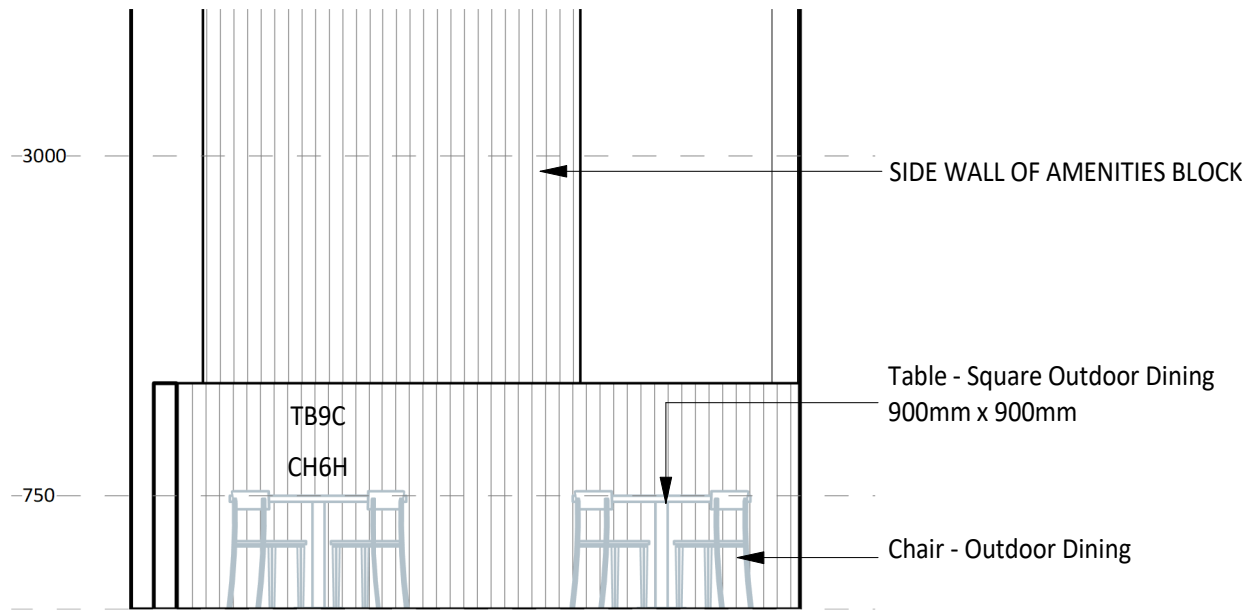
2 ELEVATION DETAIL 60-002 1 : 50
