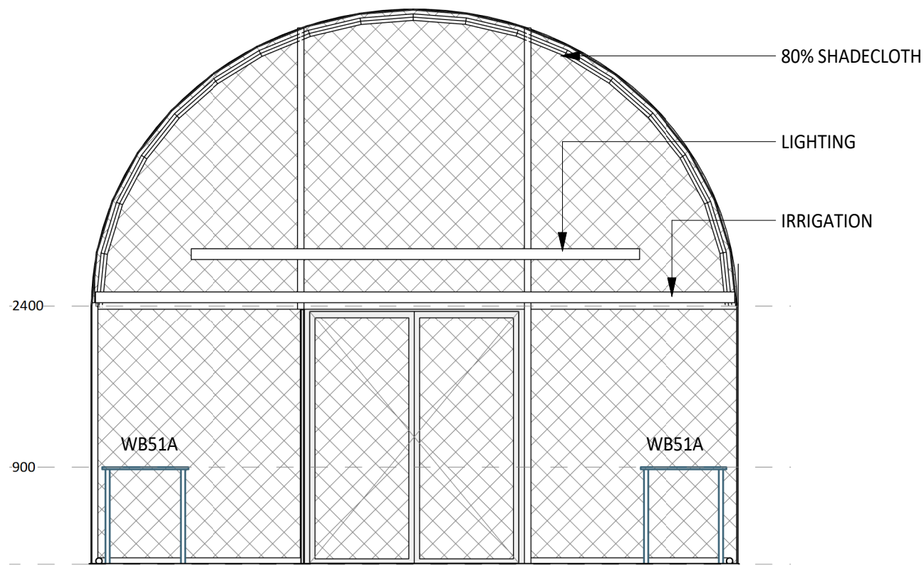
2 ELEVATION DETAIL 60-007 1 : 50
