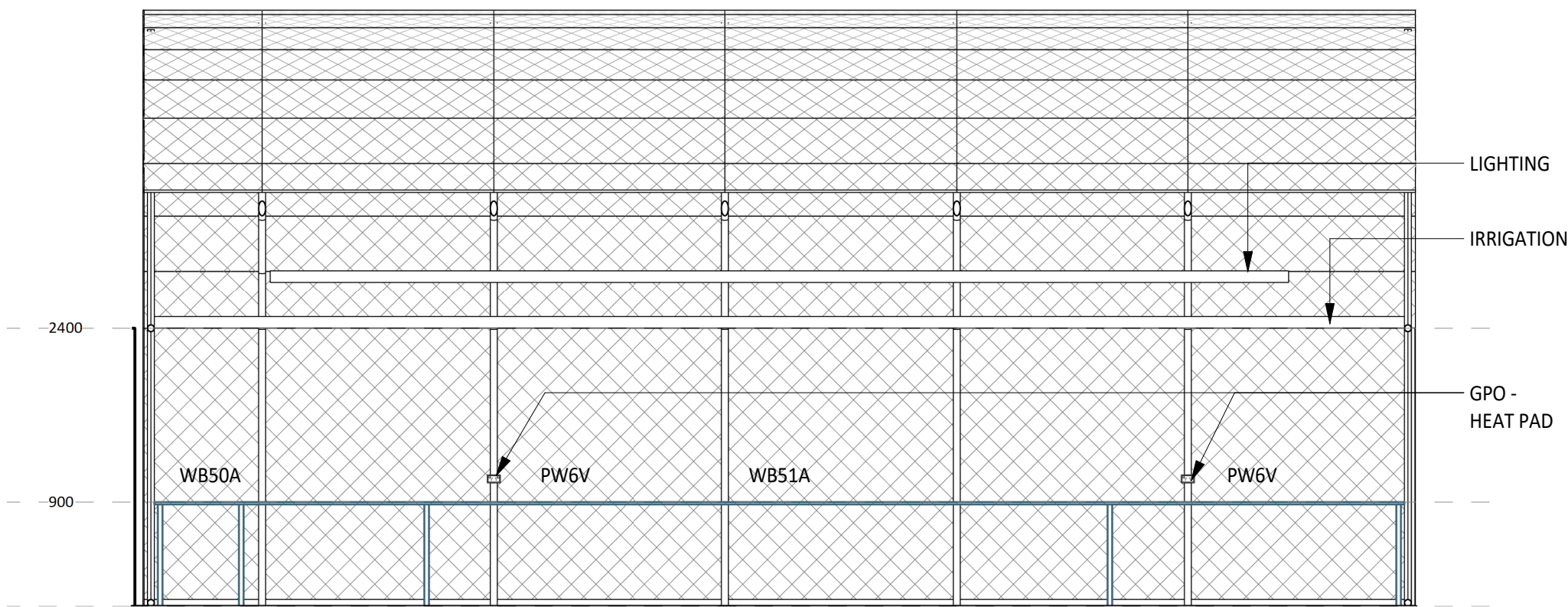
3 ELEVATION DETAIL 60-003 1 : 50
