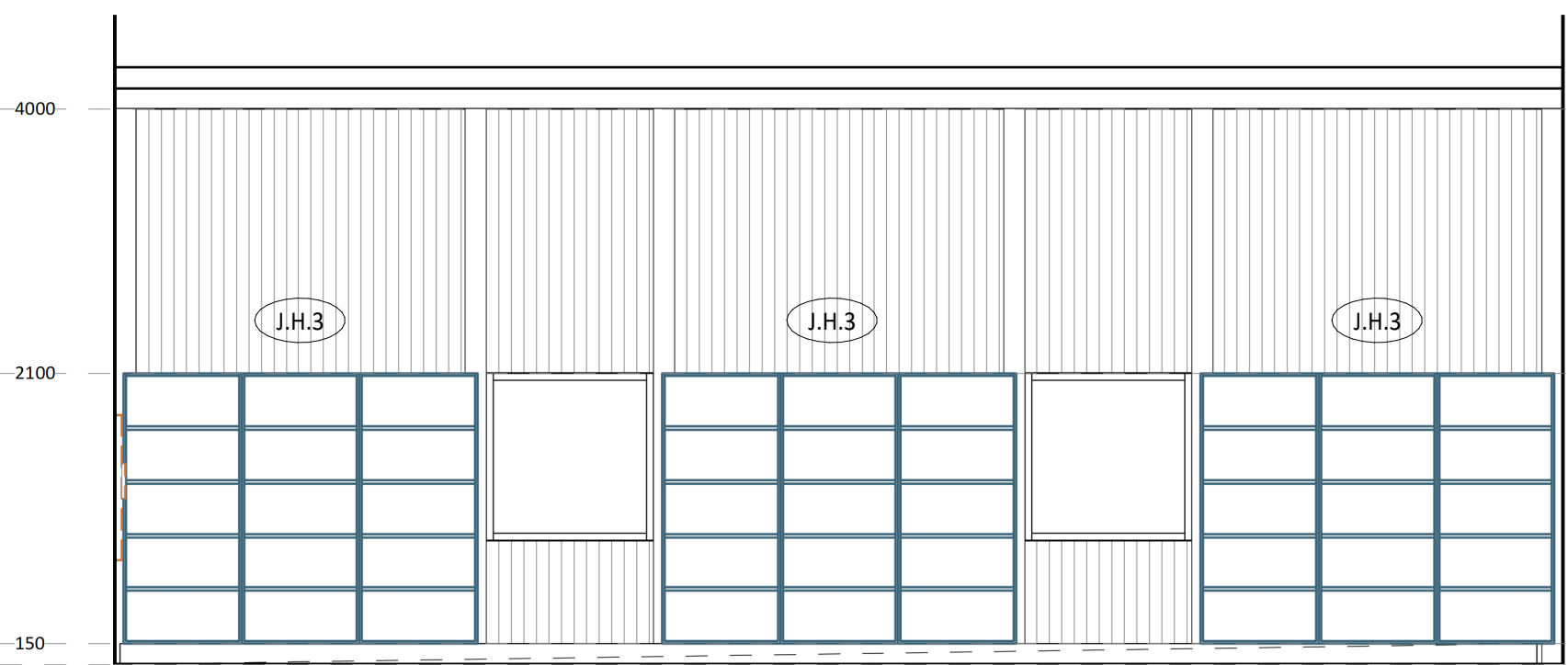
5 ELEVATION DETAIL 60-003 1 : 50
