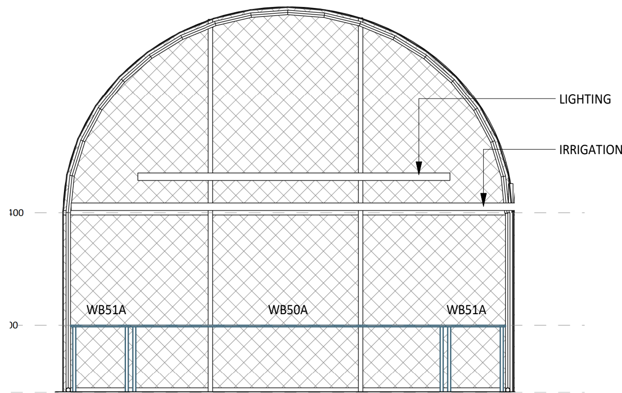
4 ELEVATION DETAIL 60-004 1 : 50
