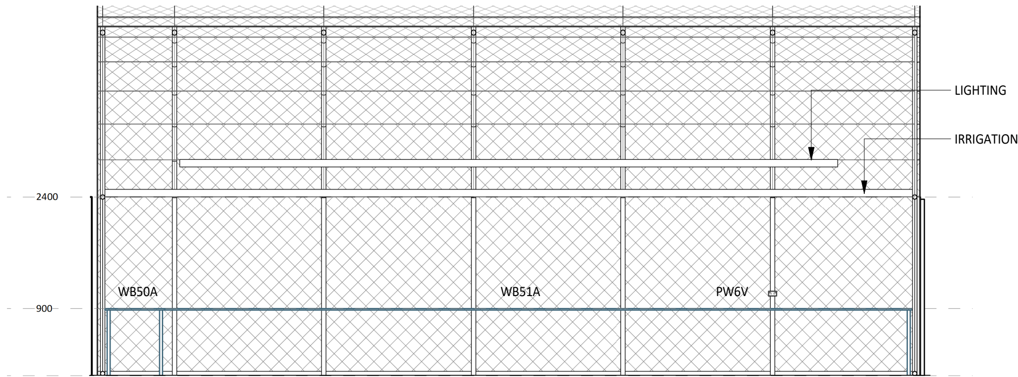
3 ELEVATION DETAIL 60-007 1 : 50
