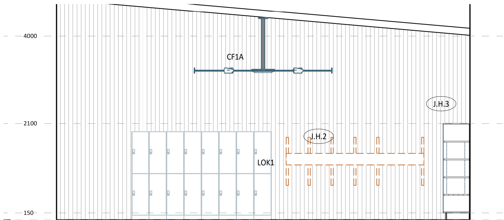
4 ELEVATION DETAIL 60-003 1 : 50
