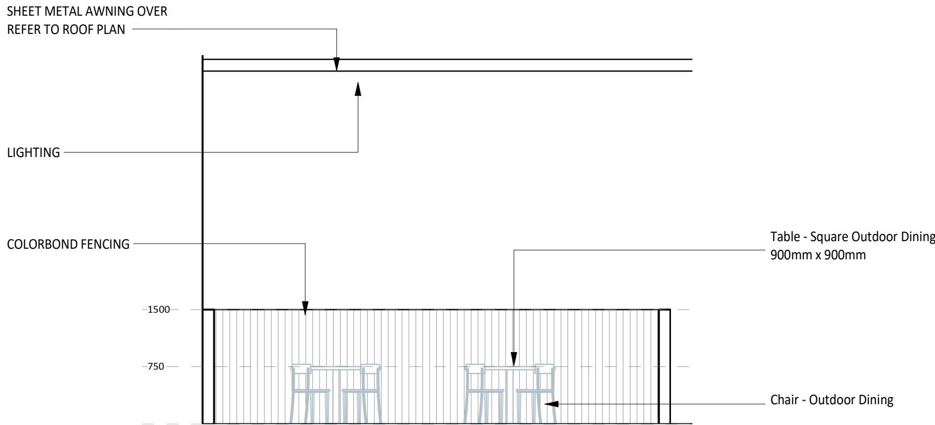
3 ELEVATION DETAIL 60-002 1 : 50
