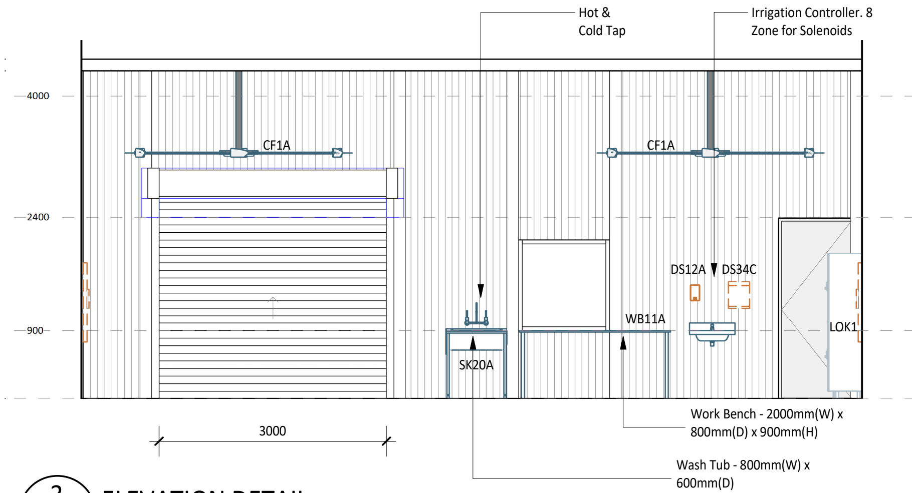
3 ELEVATION DETAIL 60-003 1 : 50
